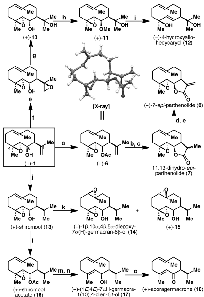
Scheme 3. Synthesis of germacrane-type sesquiterpenes. Reagents and conditions: a) DCC (3 equiv), DMAP (0.5 equiv), AcOH (3 equiv), CH 2 Cl 2 , RT, quant.; b) 9-BBN (2 equiv), THF, RT, 2 h, then EtOH, 6 h aq. NaOH, 35% aq. H 2 O 2 ; c) TEMPO (0.5 equiv), PhI(OAc) 2 (4 equiv), CH 2 Cl 2 , RT, 4 h, 77% over 2 steps; d) LDA (3.6 equiv), THF, −78°C, 1 h, then CBr 4 (4 equiv), 0.5 h; e) TBAF (3 equiv), THF, RT, 1 h, 60% over 2 steps; f) VO(acac) 2 (0.27 equiv), TBHP (2.2 equiv), CH 2 Cl 2 , 0°C, 77%; g) LiAlH 4 (5 equiv), THF, 0°C, 20 min; h) MeSO 3 Cl (3 equiv, as 2 portions), Et 3 N (3 equiv, as 2 portions), CH 2 Cl 2 , −5°C, 0.5 h, 44% over 2 steps; i) lithium naphthalenide (10 equiv, as 2 portions), THF, −25°C, 20 min, 65% of 12 , 23% of 10 ; j) Crabtree's cat. (7.5 mol%), 2,6-di- tert -butylpyridine (1 equiv), CH 2 Cl 2 , H 2 (1 atm), RT, 1 h, 65–84%; k) m CPBA (1.5 equiv), NaHCO 3 (2 equiv), CH 2 Cl 2 , −5°C, 30 min, 62% of 14 , 22% of 15 ; l) DCC (3 equiv), AcOH (3 equiv), DMAP (0.5 equiv), CH 2 Cl 2 , RT, 2 h, quant.; m) WCl 6 (1.85 equiv), n BuLi (3.8 equiv), THF, −60°C to RT, 86%; n) K 2 CO 3 (10 equiv), MeOH, 50°C, 1 h, 95%; o) IBX (4 equiv), DMSO, RT, 2 h, 90%. DCC = N,N' -dicyclohexylcarbodiimide, DMAP = 4-dimethylaminopyridine, BBN = borabicyclo[3.3.1]nonane, TEMPO = (2,2,6,6-tetramethylpiperidin-1-yl)oxyl, LDA = lithium diisopropylamide, TBAF = tetra- n -butylammonium fluoride, TBHP = tert -butyl hydroperoxide, m CPBA = meta -chloroperbenzoic acid, IBX = 2-iodoxybenzoic acid.
